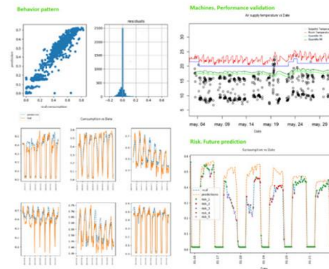
Incidence prediction models based on ML and statistical techniques
